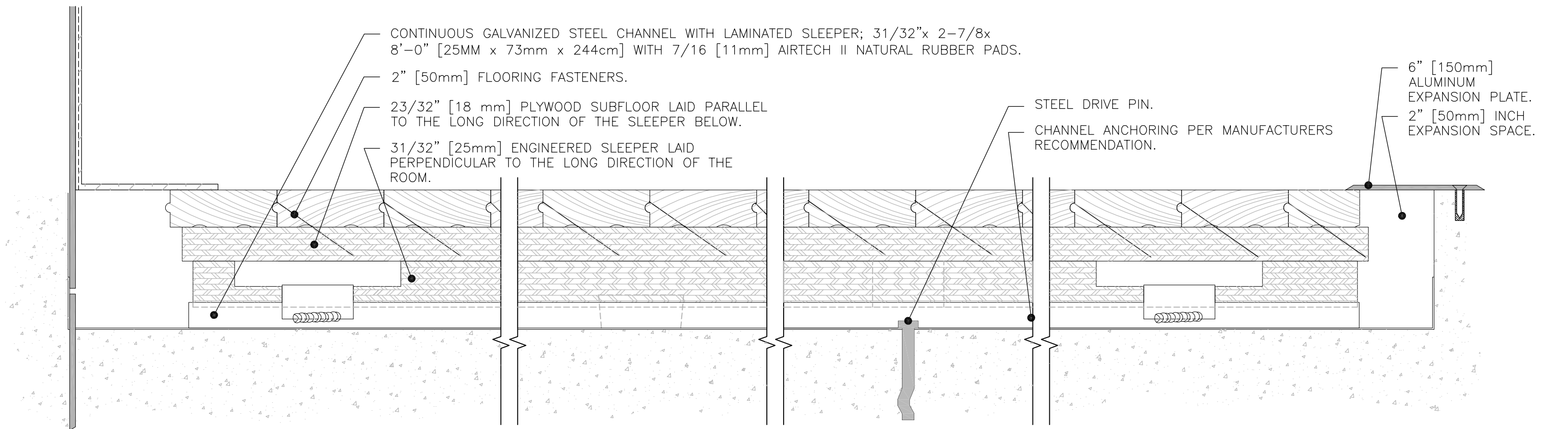
Action_PowerChannel Section across room width
