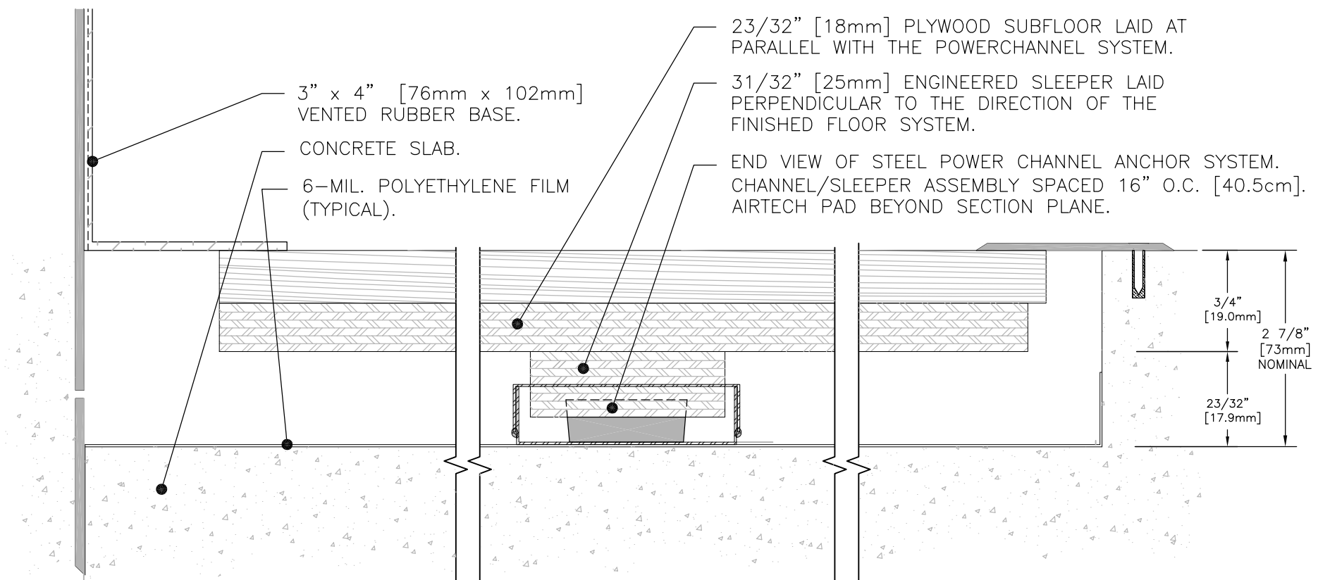
Action_PowerChannel Section across room length
